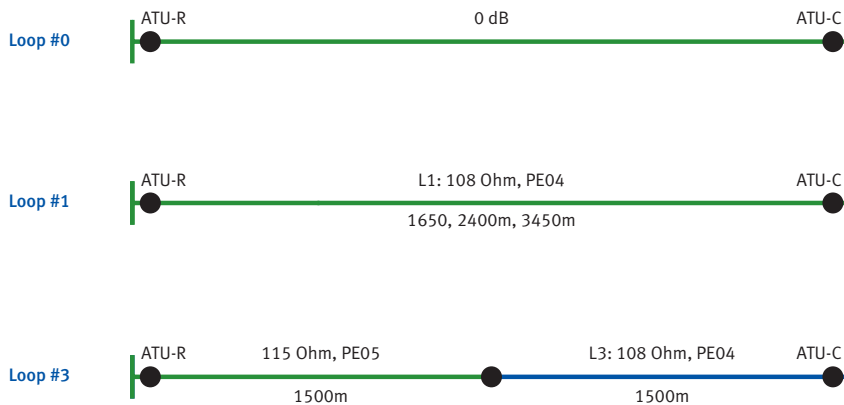
Figure 1: Proposed G.adslplus Annex G test loop topologies
